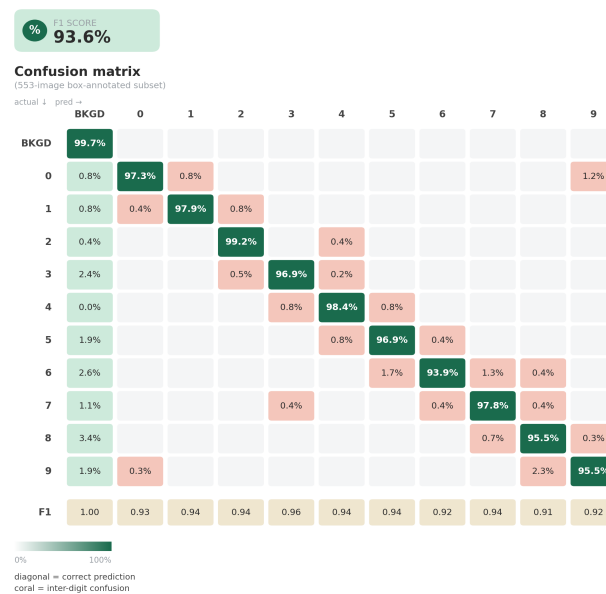
Figure 5. Row-normalised confusion matrix of the INT8 model on the 553-image box-annotated test subset
