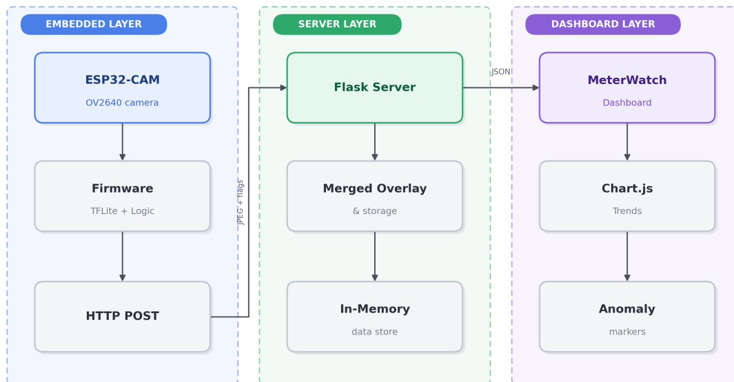
Figure 3. System architecture connecting the ESP32-CAM, the Flask server, and the MeterWatch dashboard
