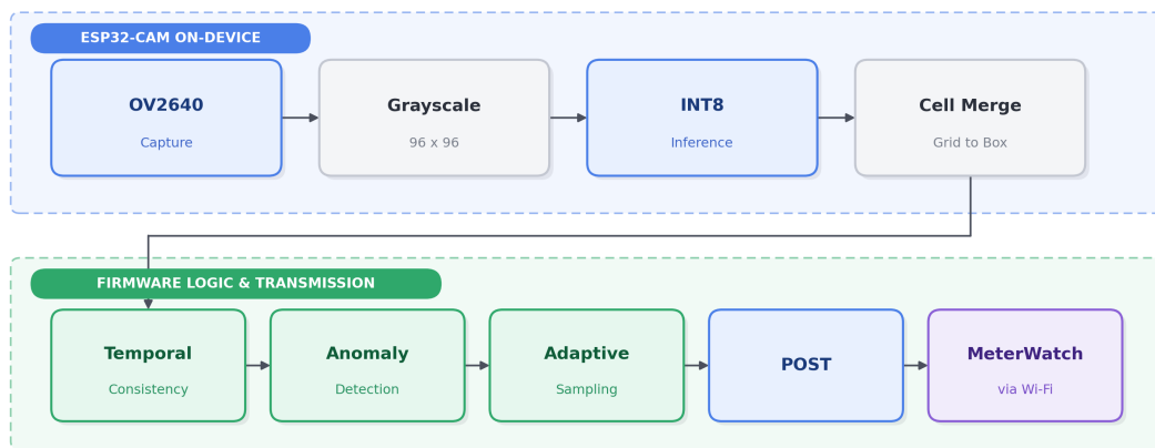
Figure 1. End-to-end system pipeline with all inference and firmware logic executed on the ESP32-CAM
