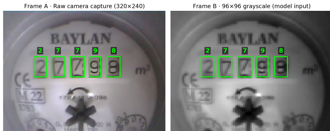
Figure 7. Preprocessing pipeline for a representative test frame
