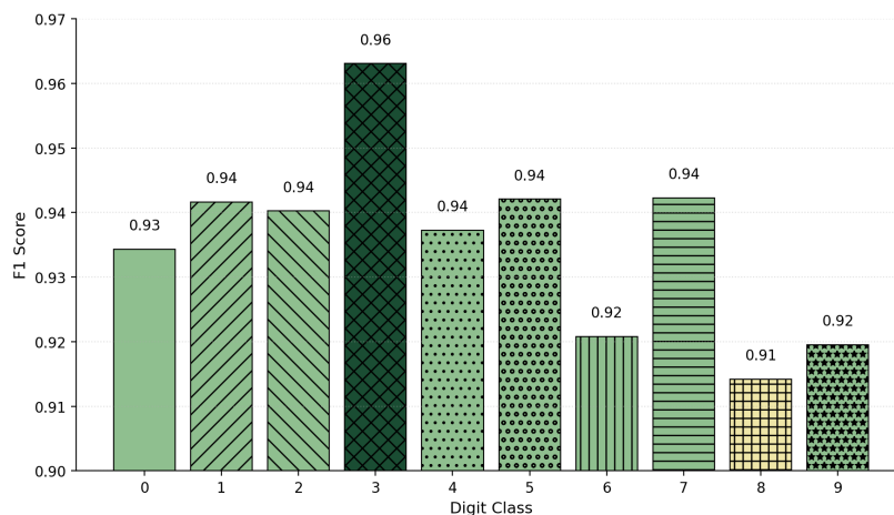
Figure 6. Per-class F1-score of the INT8 model across the ten digit classes
