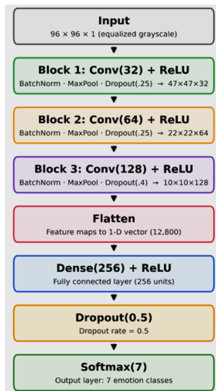
Figure 2. Architecture of the lightweight CNN used for emotion classification
