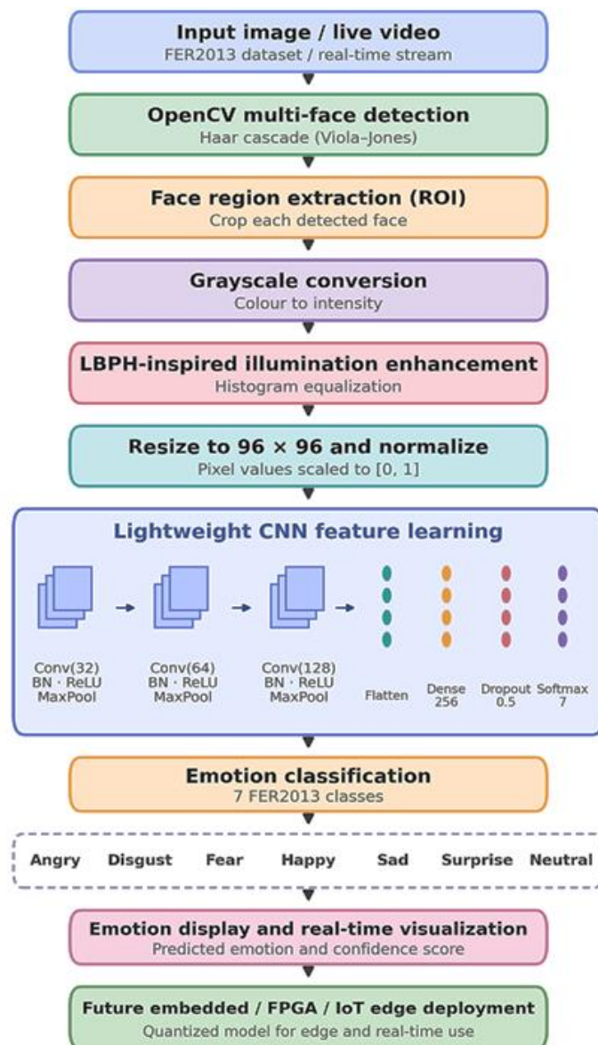
Figure 1. Overall workflow of the proposed hybrid LBPH-inspired CNN framework for interactive web interface-based multi-face emotion recognition
