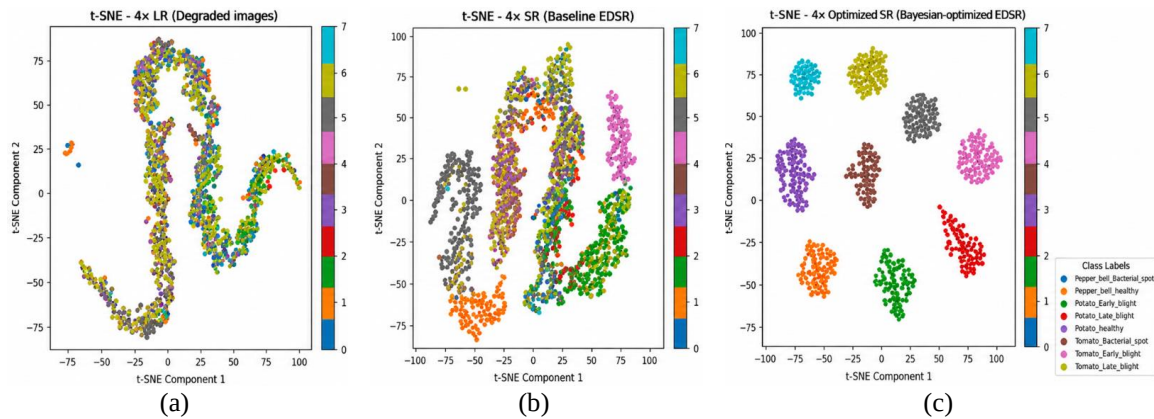
Figure 3. t-SNE visualization of lesion-aware Color GLCM feature distributions for: (a) 4× degraded LR images, (b) baseline EDSR reconstructed images, and (c) Bayesian-optimized EDSR reconstructed images, with the axes representing the first and second t-SNE embedding dimensions and the colors denoting the eight disease classes
