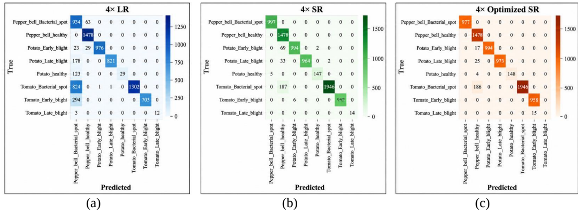
Figure 2. Confusion matrices for disease classification under different image-resolution conditions: (a) 4× degraded LR images, (b) baseline EDSR reconstructed images, and (c) Bayesian-optimized EDSR reconstructed images
