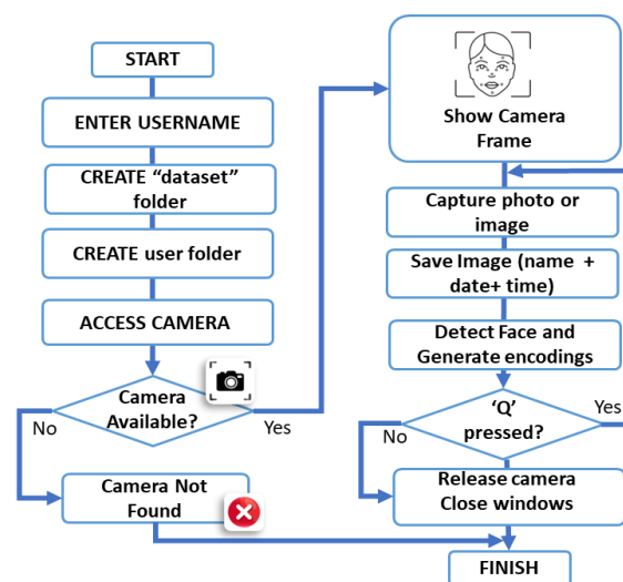
Figure 2. Flowchart for registering a new user
