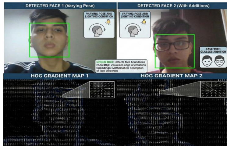
Figure 9. Face detection using the HOG method
