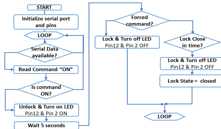
Figure 5. Programming flowchart for the ESP32
