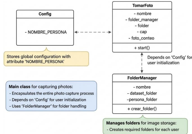
Figure 3. Class diagram for user registration
