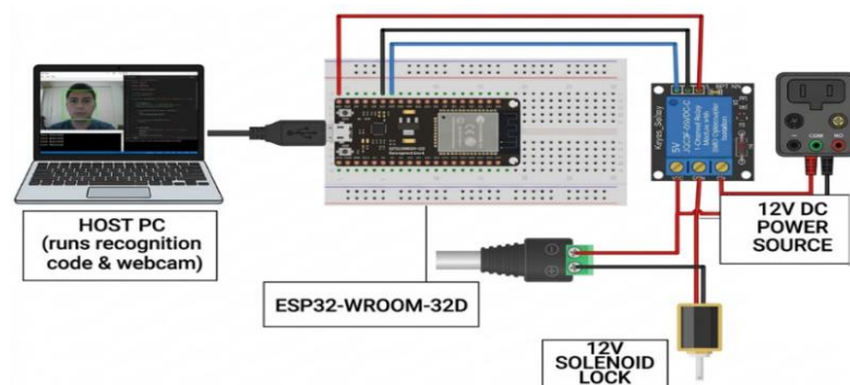
Figure 6. Circuit interconnection diagram
