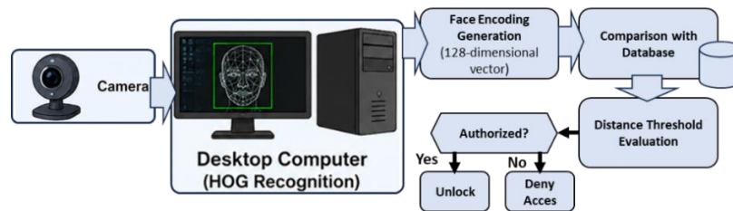
Figure 4. Facial recognition workflow
