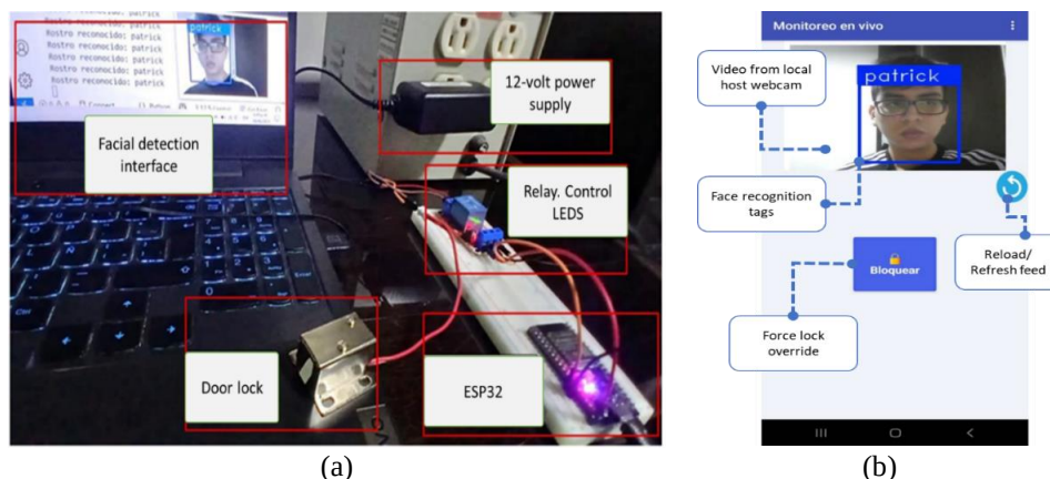
Figure 11. Validation of the control program's functionality with ESP32 using; (a) implemented physical circuit and (b) remote monitoring with the mobile app
