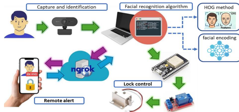
Figure 1. Project component diagram
