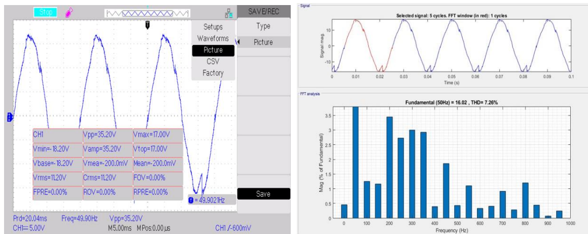
Figure 4. Experimental AC output for the 27-level TSLMLI with 2 errors induced at S_1 and B_1 and its THD% as 7.26%
