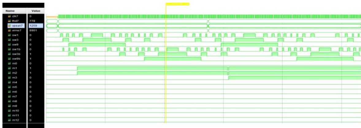
Figure 6. Output for the prediction of the KNN algorithm using inverter parameters of THD%, V_{RMS} , and V_{PEAK}
