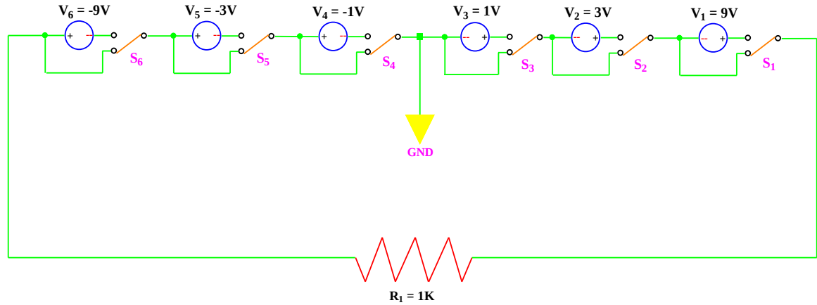
Figure 1. TSLMLI circuit topology
