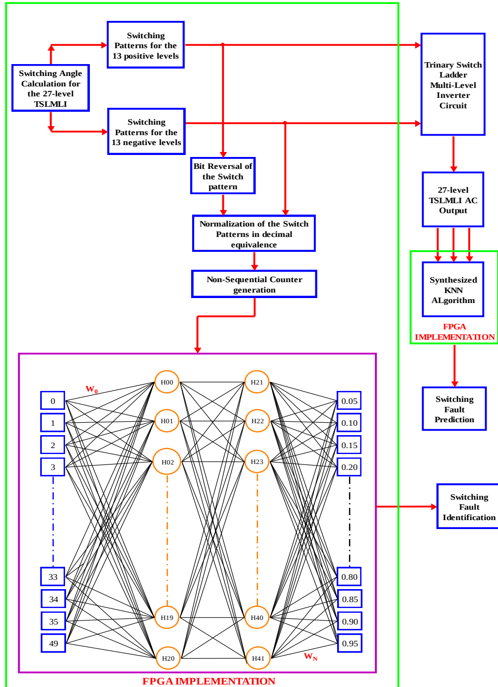
Figure 2. Block diagram of the proposed switch pattern algorithm to fault occurrence in the 27-level TSLMLI
