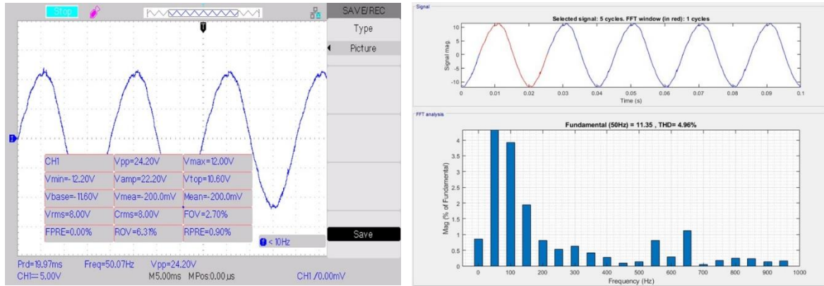
Figure 3. Experimental AC output for the 27-level TSLMLI without any error induction with THD% as 4.96%
