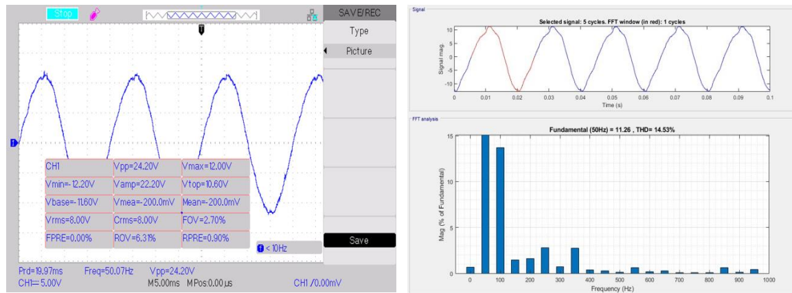
Figure 5. Experimental AC output for the 27-level TSLMLI with 2 errors induced at S_3 and B_1 and its THD% as 14.53%
