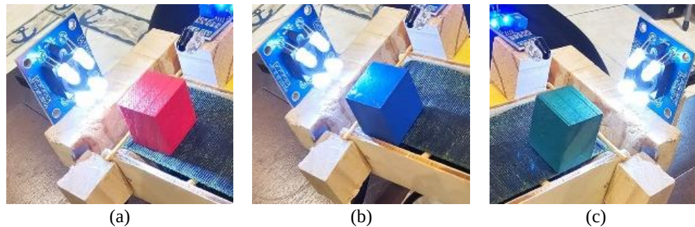
Figure 6. Setup showing the colour sensor facing different coloured objects: (a) red colour detection, (b) blue colour detection, and (c) green colour detection
