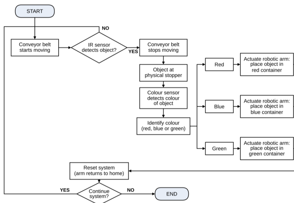
Figure 3. Block diagram
