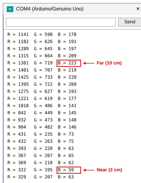
Figure 5. Raw frequency data from colour sensor when a blue object is placed at different distances
