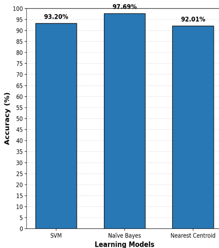
Figure 3. Evaluation of ML algorithms' performances
