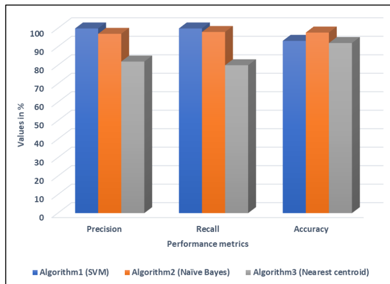
Figure 5. Comparison of precision, recall, and accuracy of the supervised learning models
