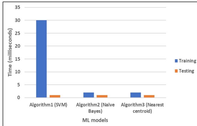
Figure 4. Training and testing time
