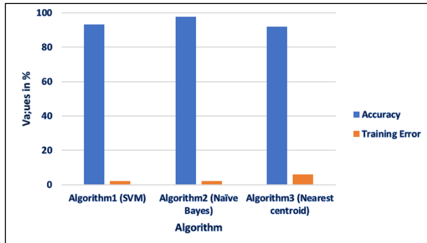
Figure 2. Effectiveness of categorizing network traffic
