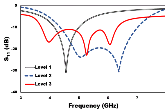
Figure 4. The evolution stages of simulated reflection coefficient ( S_{11} )
