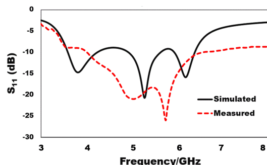
Figure 6. Comparison graph of S-parameter of the proposed antenna in both simulation and measurement
