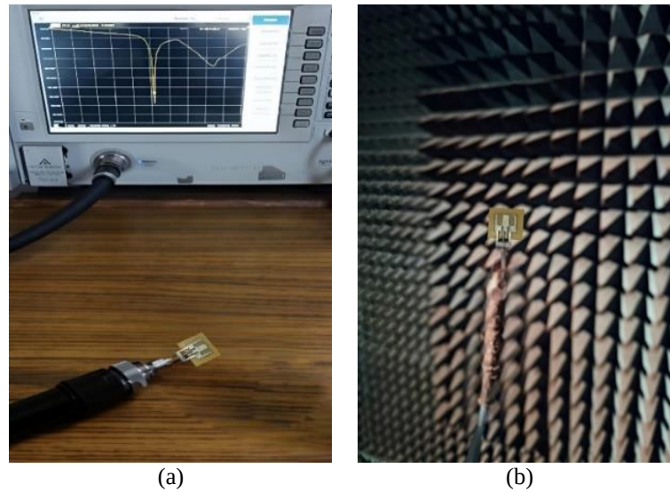
Figure 5. Antenna measurement setups used for performance validation; (a) reflection coefficient measurement with a VNA and (b) radiation pattern assessment in an anechoic environment
