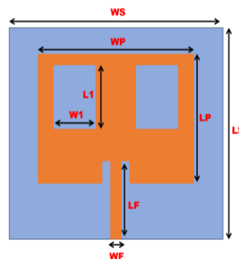
Figure 2. Total geometry and configuration of the proposed antenna
