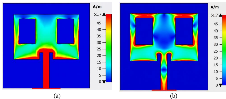
Figure 8. Surface current density of the proposed grid array antenna; (a) 3.6 GHz and (b) 6.2 GHz
