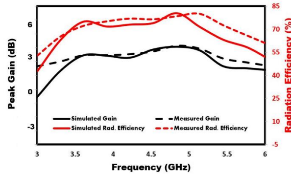
Figure 10. Variation in the designed slotted antenna's peak gain and radiation efficiency
