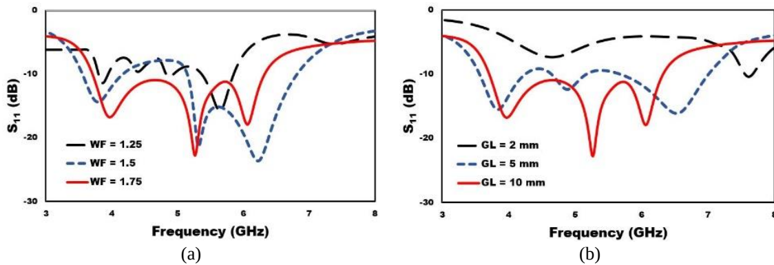
Figure 7. Reflection coefficients under different operating conditions; (a) parametric study of feed width and (b) GL
