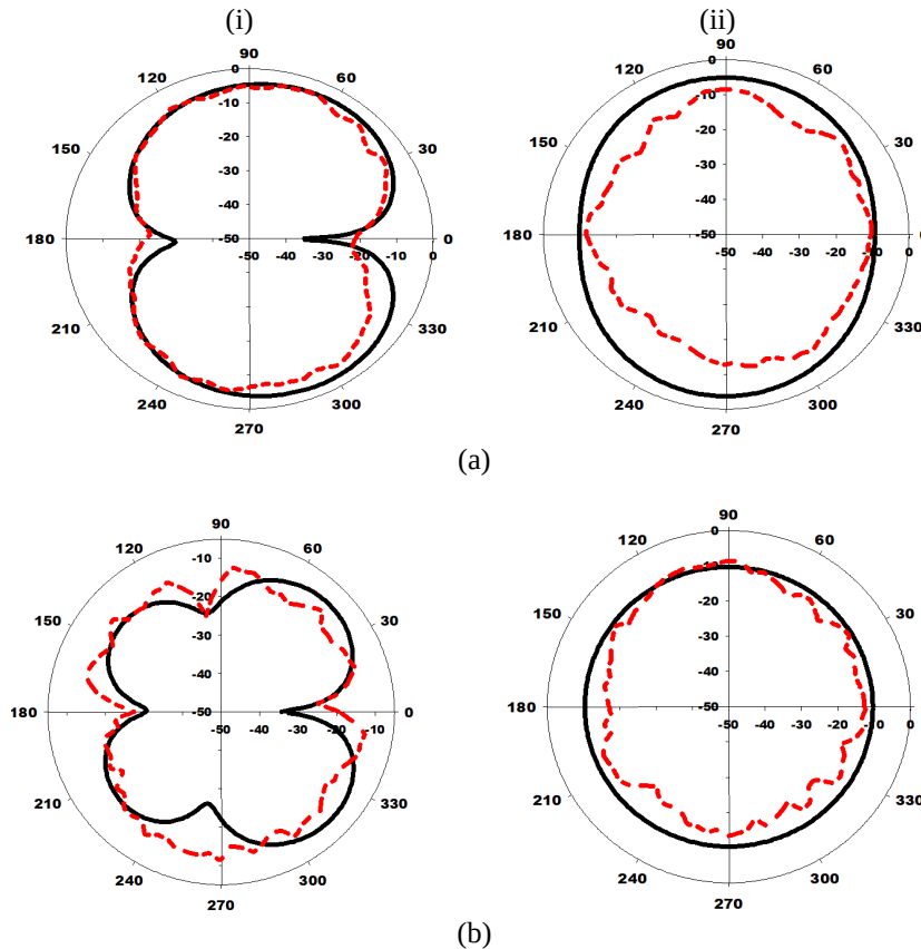
Figure 9. Measured and simulated 2D radiation pattern results of the antenna in the (i) E-plane and (ii) H-plane at frequencies of; (a) 3.6 GHz and (b) 6.2 GHz
