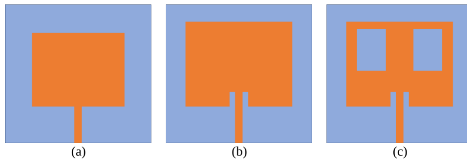
Figure 3. Step-by-step evolution; (a) initial structure (Level 1), (b) intermediate structure (Level 2), and (c) final structure (Level 3)
