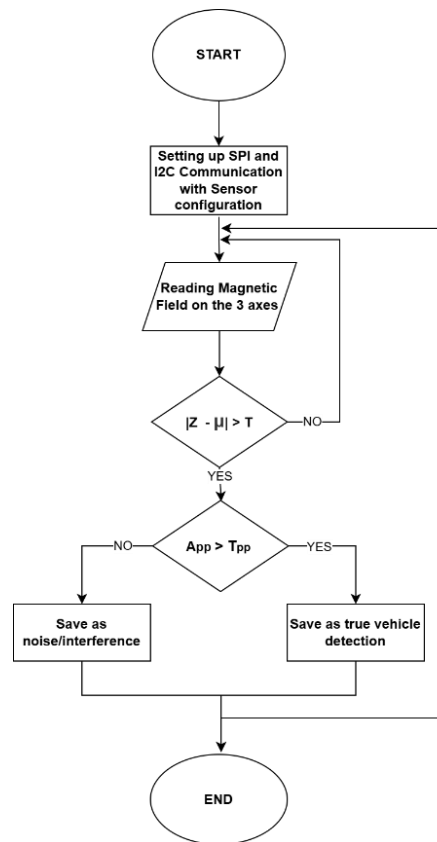
Figure 5. Vehicle detection flowchart
