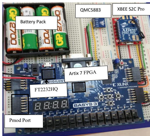
Figure 3. Sensor node components
