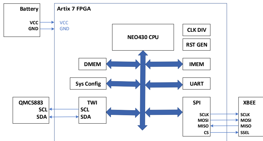
Figure 2. Sensor node architecture
