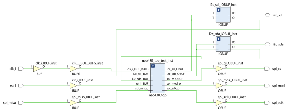
Figure 6. Schematic diagram of the on-chip system of the traffic detection unit
