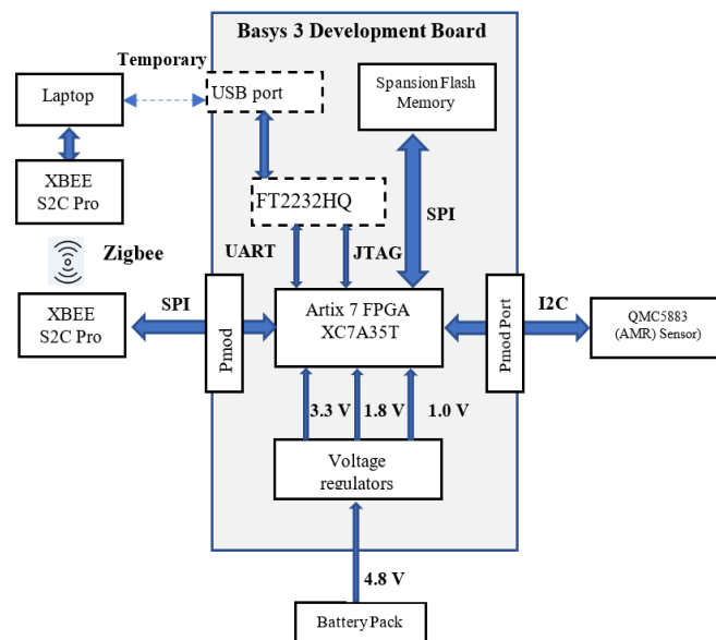
Figure 1. Sensor node design block diagram
