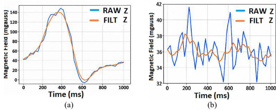
Figure 8. Magnetic signatures of: (a) valid car passage and (b) rejected noise signal
