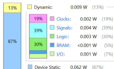
Figure 7. On-chip power consumption
