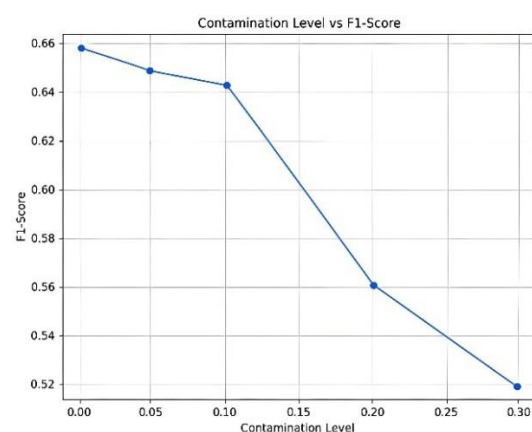
Figure 5. Graphical analysis of contamination level and F1-score
