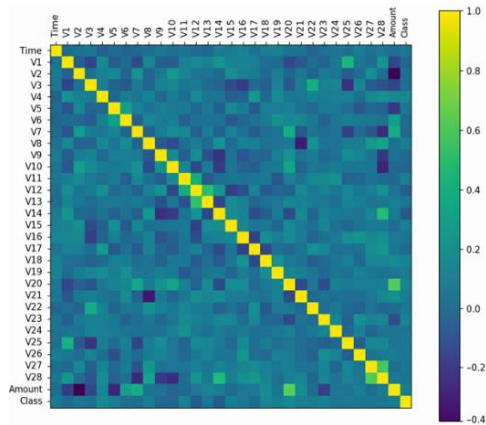
Figure 2. Correlation matrix
