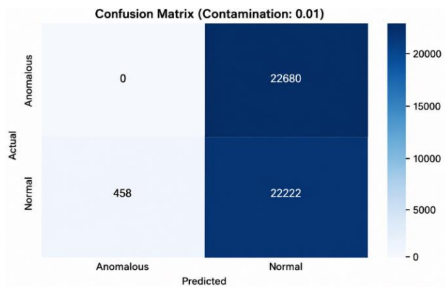
Figure 3. Confusion matrix
