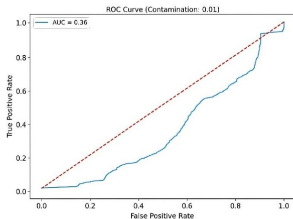
Figure 4. ROC curve
