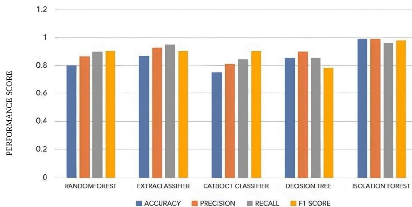
Figure 6. Comparison graph between existing and proposed algorithm
