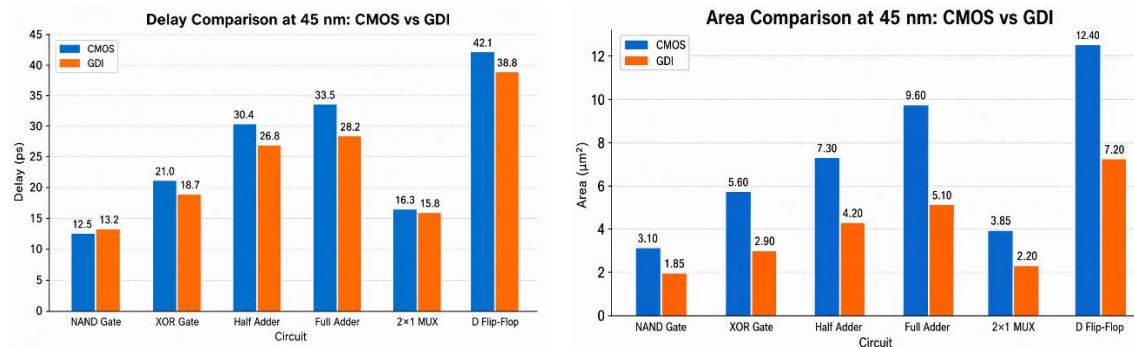
Figure 3. Comparison of CMOS and GDI implementations at 45 nm; (a) propagation delay and (b) silicon area
