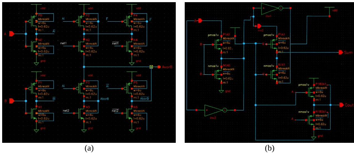
Figure 2. Representative transistor-level schematics implemented in 45 nm technology; (a) CMOS XOR gate and (b) CMOS full adder
