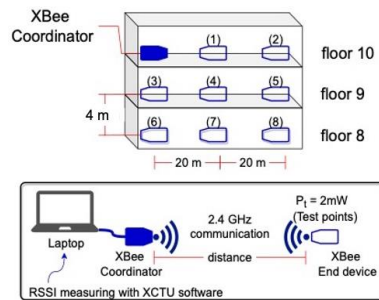
Figure 5. Schematic diagram of ZigBee test setup with RSSI measurement using XCTU software
